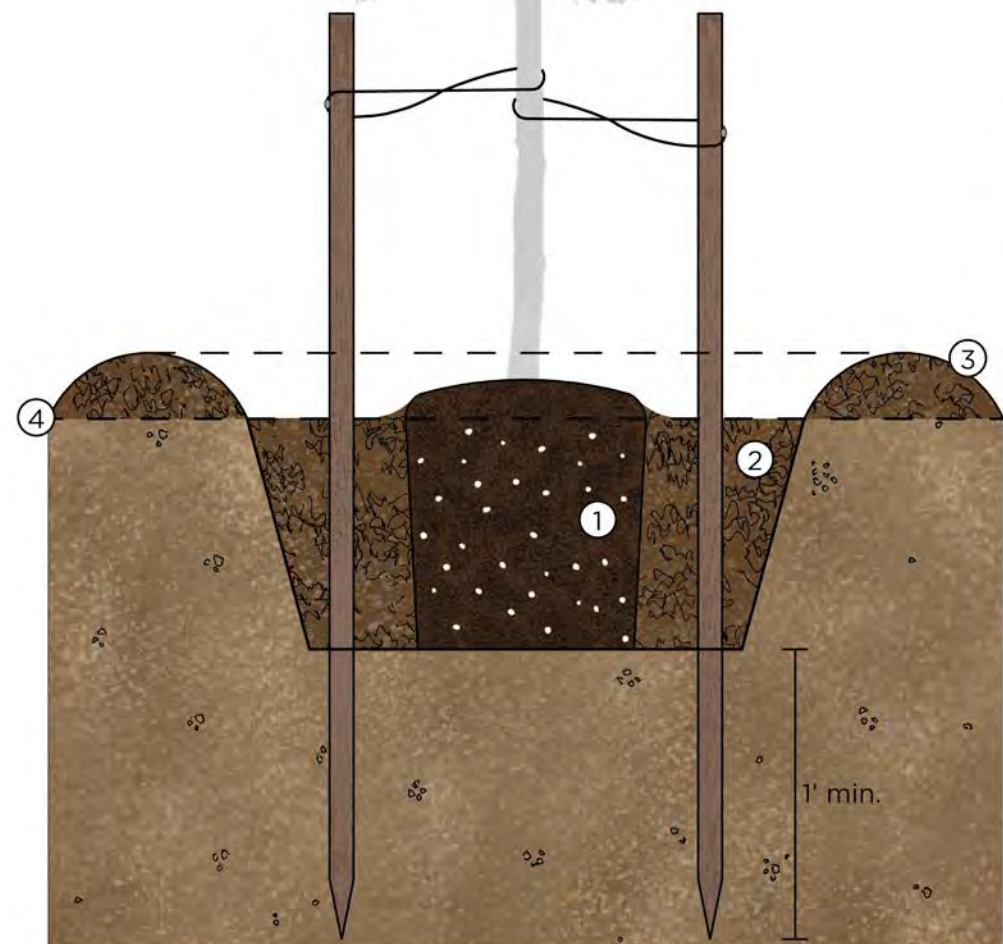
PLANTING DETAIL 5 AND 15 GALLON TREES
