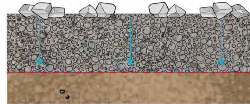
FRENCH DRAIN LEVEL BOTTOM
